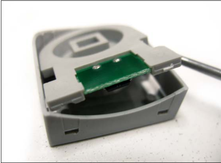
26. Carefully lift the chip from its housing.
