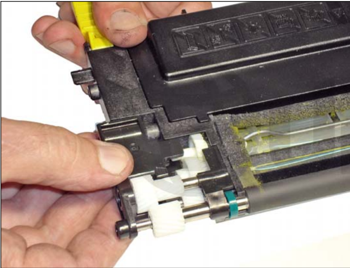
14. Install the gear cover making sure the gears fit properly on their respective shafts.
