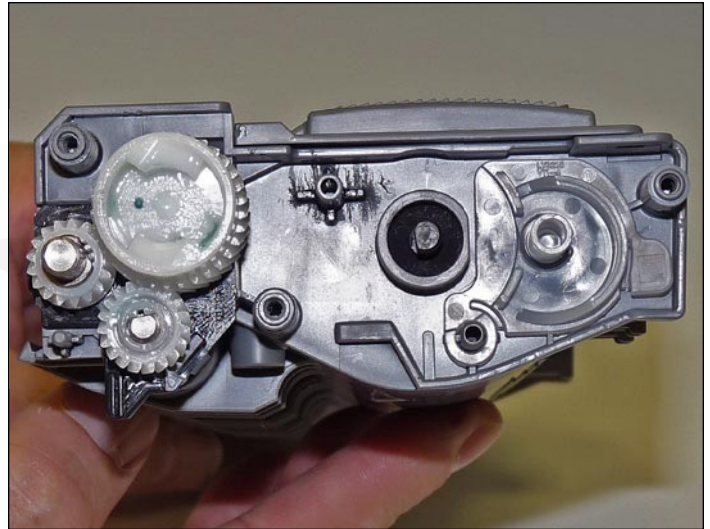
17. Install the E-ring on the developer roller shaft.
